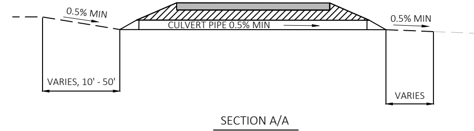
DRIVEWAY CULVERTS
