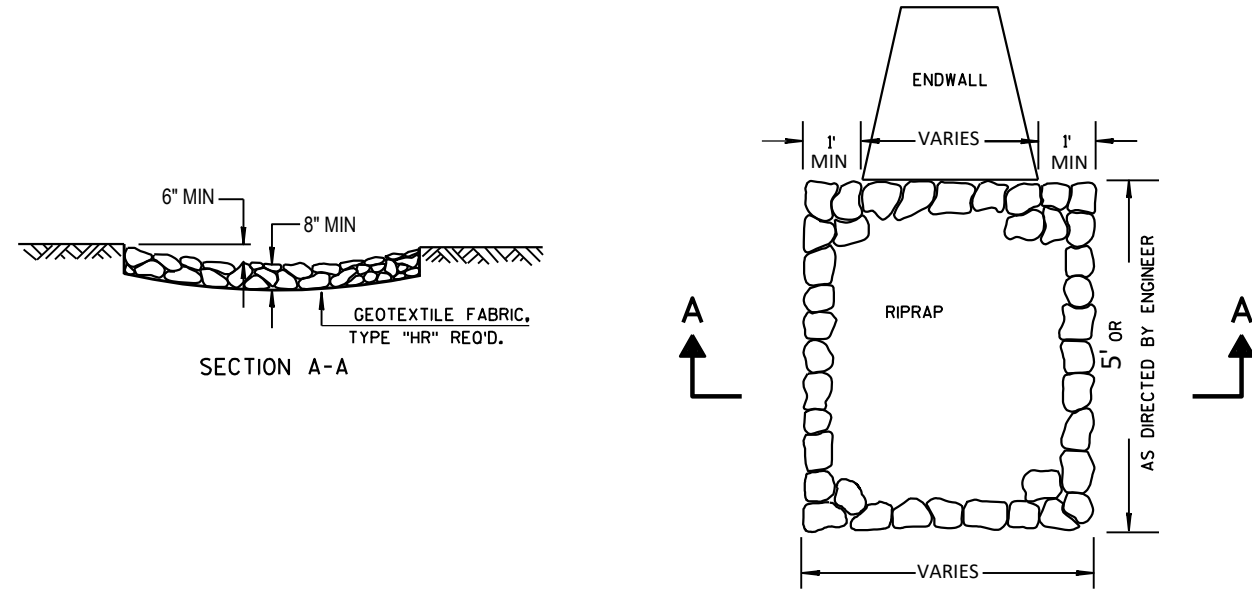
RIPRAP TREATMENT AT APRON ENDWALL (OPTIONAL)
